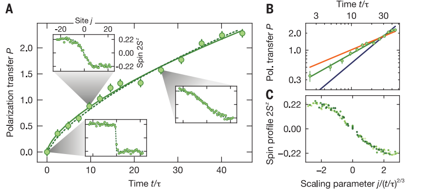
Fig. 2. Superdiffusive spin transport in a high-temperature Heisenberg chain. (A) The polarization transfer for a domain-wall initial state with a contrast of \eta = 0.22(2) grows as a power law [ P(t) \propto t^{1/z} ] with a fitted exponent z = 1.54(7) (solid line), indicating superdiffusive transport. The experimental data are consistent with numerical Heisenberg-model simulations (41) (dashed line). The insets show the averaged spin profiles 2S_j^z(t) at times t/\tau = 0, 10, 26 , which are compared to simulations (dashed lines). (B) Polarization transfer in a double-logarithmic plot. The solid lines are power-law fits with fixed exponents, where a distinction between z = 3/2 (green) and both z = 2 (brown) and z = 1 (blue) is visible. (C) When rescaling time by the inverse dynamical exponent, the spatial spin profiles at times t/\tau = 5 to 35 (light to dark green) collapse to a characteristic shape consistent with the integrated KPZ function. Error bars denote SEM.
