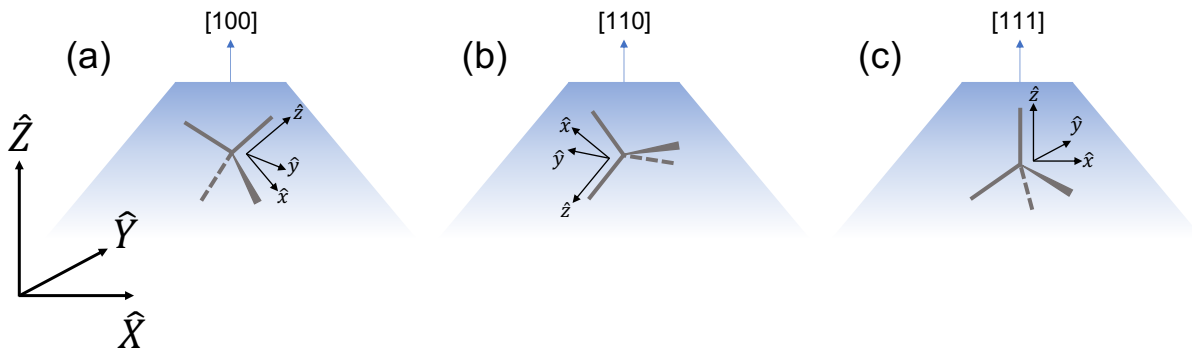
Figure 2.8: Crystal cut of culet [75] : The three main crystal cuts for diamond anvils are shown along with the orientation of the four NV groups therein. As a convention in this thesis, \{\hat{X}, \hat{Y}, \hat{Z}\} represents the lab frame, whereas \{\hat{x}, \hat{y}, \hat{z}\} represents the reference frame of a single NV group. The \hat{Z} axis in the lab frame is the loading axis in all cases. In each case, the local frame \{\hat{x}, \hat{y}, \hat{z}\} of one of the NV groups is shown. (a) In a [100] cut anvil, the four NV groups are degenerate with respect to the loading axis. (b) In a [110] cut anvil, two sets of NV groups are each doubly degenerate with respect to the loading axis. One set is oriented in the plane of the culet, whereas another set projects strongly on the loading axis. (c) In a [111] cut culet, one NV group is fully oriented along the loading axis. Note that the local frame of this [111] NV group is coincident with the lab frame. The other three NV groups are degenerate with respect to the loading axis.
