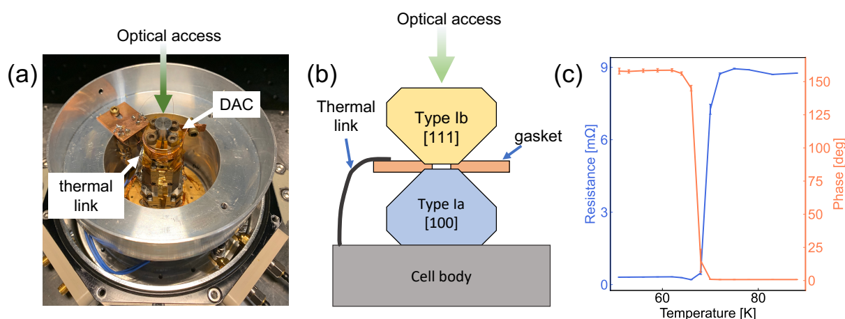
Figure 7.6: Thermal linking: (a) A custom thermal link (Four Nine Design) between the cell body and the cold finger of the cryostat allowed for better thermalization. The thermal link was secured to the cell body using a girdle machined out of a copper plate. (b) A second thermal link was attached between the metal gasket and the cell body to account for the diminishing thermal conductivity of diamond below 100 K. The link was cut out from Indium (In) foil and attached at either end by cryogenic epoxy (Stycast ® 2850FT). (c) Lock-in measurements show a drop in sample resistance at \sim 70 K at zero applied magnetic field. This resistance drop is accompanied by a jump in the measured phase from 0^\circ to \sim 150^\circ deep in the superconducting state. The transition point is \sim 20 K lower than the true T_C of the sample due to the thermal gradient between the cold finger (location of temperature reading) and the high pressure sample.
