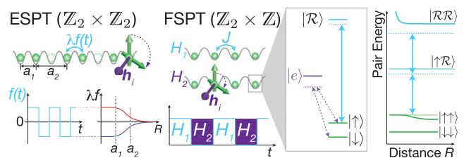
FIG. 1. A 1D array of atoms is trapped in an optical lattice or tweezer array. Ising interactions for pseudospin states |\downarrow\rangle , |\uparrow\rangle are generated by optically coupling |\uparrow\rangle to Rydberg state |\mathcal{R}\rangle (solid blue arrows). Random fields h_i are generated by a spatially varying Raman coupling (dotted purple arrows) between |\downarrow\rangle and |\uparrow\rangle . While emulating the ESPT phase requires a dimerized chain with Ising couplings \lambda f(t) of dynamically switchable sign, the FSPT phase is simulated simply by alternating between two Hamiltonians consisting of Ising interactions ( H_1 ) and a disordered transverse field ( H_2 ).
