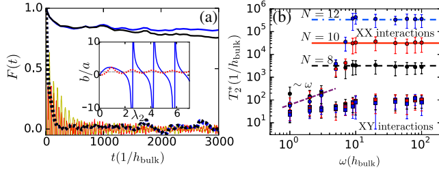
FIG. 2. ESPT phase—(a) F^\alpha(t) for N = 10 spins with \omega = 100 , V_x = 0.05 , V_y = 0 , \lambda_1 = 1.54 and \lambda_2 = 0.69 , yielding b(\lambda_1, \lambda_2)/a(\lambda_1, \lambda_2) \sim 10 . Almost overlapping dotted lines represent the clean undisordered case (black and blue for F^z and F^x , respectively). Solid lines correspond to strong on-site disorder, with thick black and blue lines for F^z and F^x in the dimerized case and thin solid yellow and red lines for F^z and F^x in the undimerized case. (inset) Ratio b(1, \lambda_2)/a(1, \lambda_2) in the dimerized (solid blue) and the undimerized (dotted red) models. The SPT phase corresponds to b/a > 1 (delimited by the dotted black line). (b) T_2^* as a function of frequency and system size [74]. As \omega is increased for V_x = 0.05 (circles), T_2^* saturates consistent with being bounded by T_2^* \sim \min(\mathcal{O}(\omega), e^{\mathcal{O}(N)}) . Adding generic interactions, V_y \sum_i \sigma_i^x \sigma_{i+1}^y with V_y = 0.2 (squares), leads to a breakdown of the edge coherence for all parameters.
