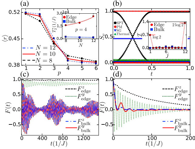
FIG. 3. FSPT phase—(a) The \langle r \rangle ratio as a function of the power law exponent p for a chain with periodic boundary conditions. The h_i 's are sampled from the uniform distribution [0.1, 0.9] and T = \pi (in units of J = 1 ). There is a MBL-delocalization phase transition around p_c \approx 3.5 . (inset) T_2^2 as a function of N , where the edge coherence is fit to \sim N^4 . (b) The entanglement spectrum micromotion for N = 12 . The parameters (p, T, J, W) are: (4, \pi, 1, 1) for the SPT; (1, \pi, 1, 1) for the thermal behavior; (4, \pi, 0.05, 0.8) for the paramagnet; p = 4, T = \pi, J = 0.5, h \in [0.5, 1] for the spin glass. (inset) Mutual information \mathcal{I}(i, j) = S_i + S_j - S_{ij} (where S is the von Neumann entropy) within the SPT phase: \mathcal{I}(1, j) (red circles) and \mathcal{I}(6, j) (blue squares) [74]. (c) F^y(t) and F^z(t) for the edge and the bulk in a system of N = 10 spins for the model in Eq. (3). The bulk curves are almost overlapping. (d) Same as in (c), but with an additional term, V_x \sum_i \sigma_i^x \sigma_{i+1}^x ( V_x = 0.3 ) added to H_1 .
